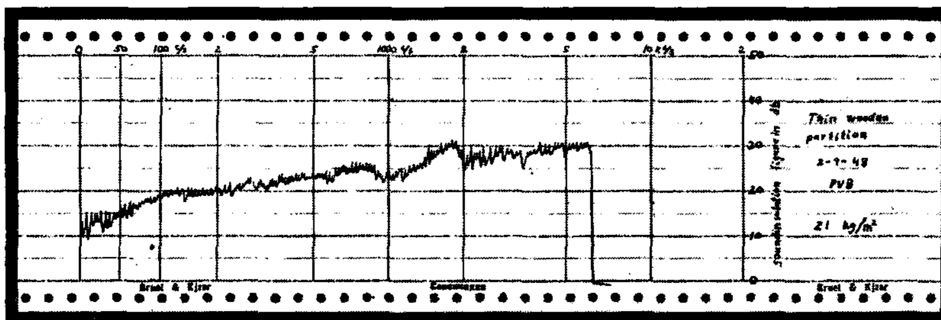
Fig. 10. Automatically recorded sound insulation curve of a thin wooden partition.
