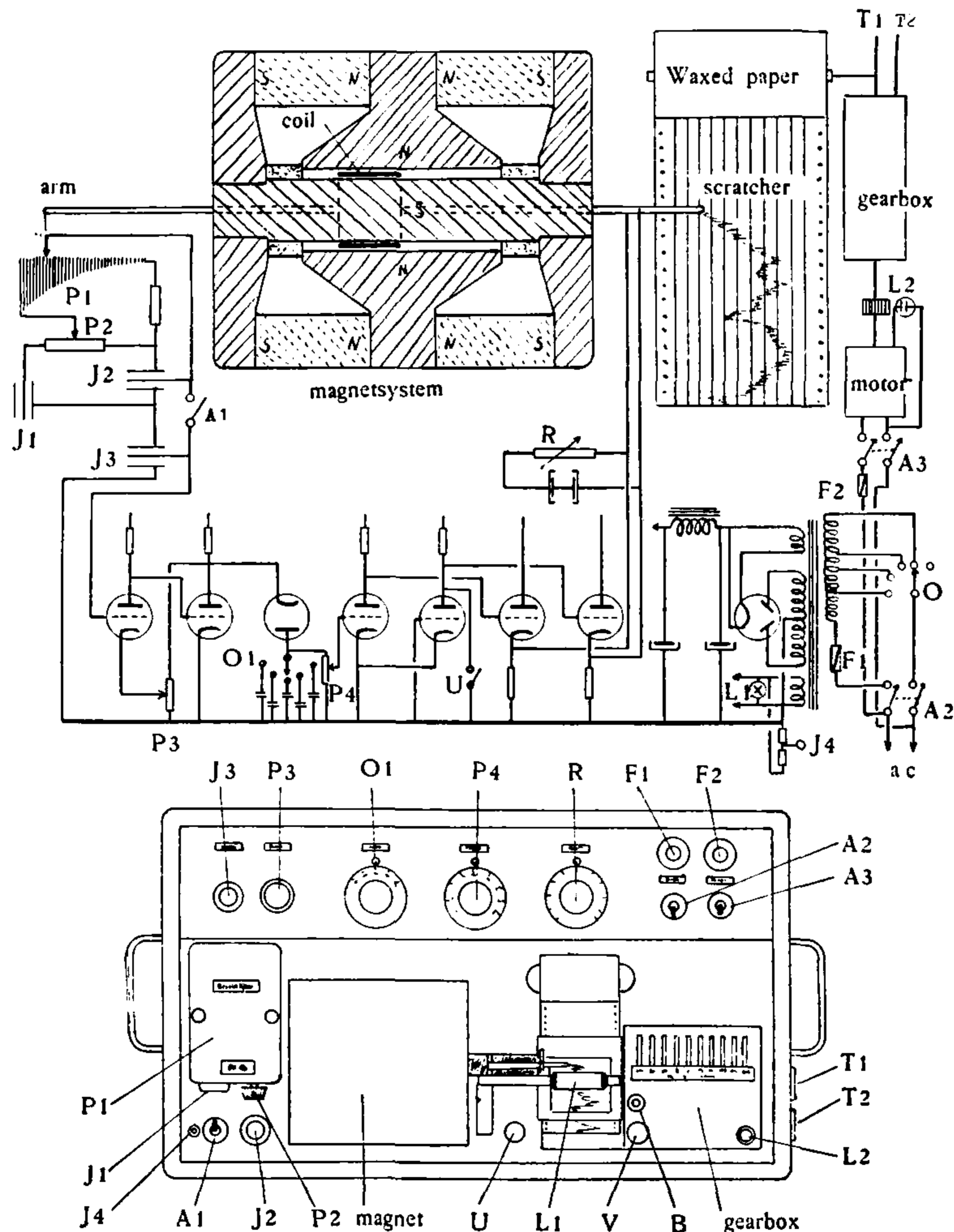
Fig. 1. Principle for the new electrodynamic recorder.
